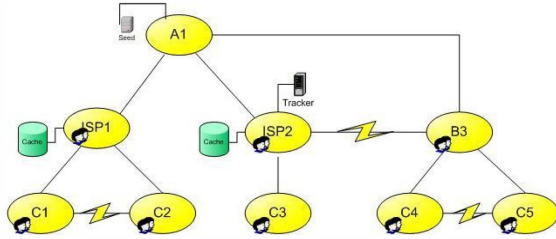
Figure 5. 9-AS topology under study.
